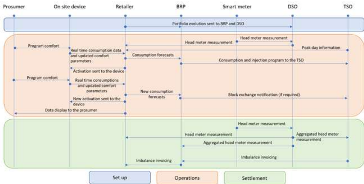
FIGURE 5 – USE CASE SEQUENCE DIAGRAM FROM THE FRENCH PILOT
