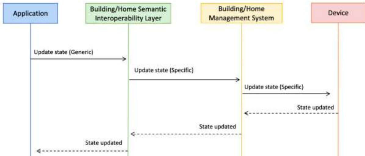
FIGURE 31 – MESSAGE FLOW EXAMPLE FOR ACTIONABLE COMMANDS FOR SPECIFIC/GENERIC MESSAGING PROTOCOLS
