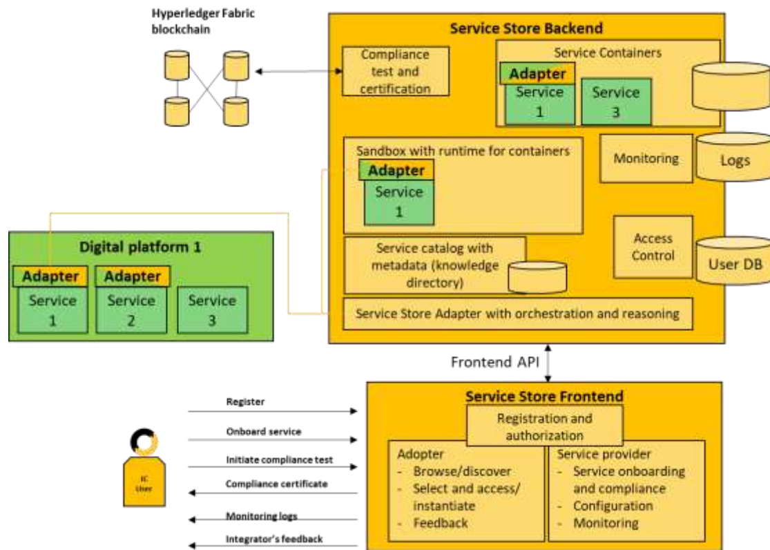
FIGURE 57 – IC'S SERVICE STORE ARCHITECTURE
