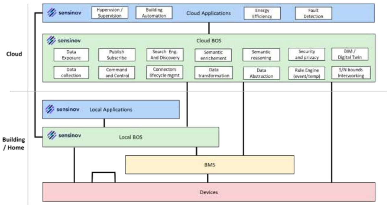
FIGURE 53 – SENSINOV’S FUNCTIONAL COMPONENTS
