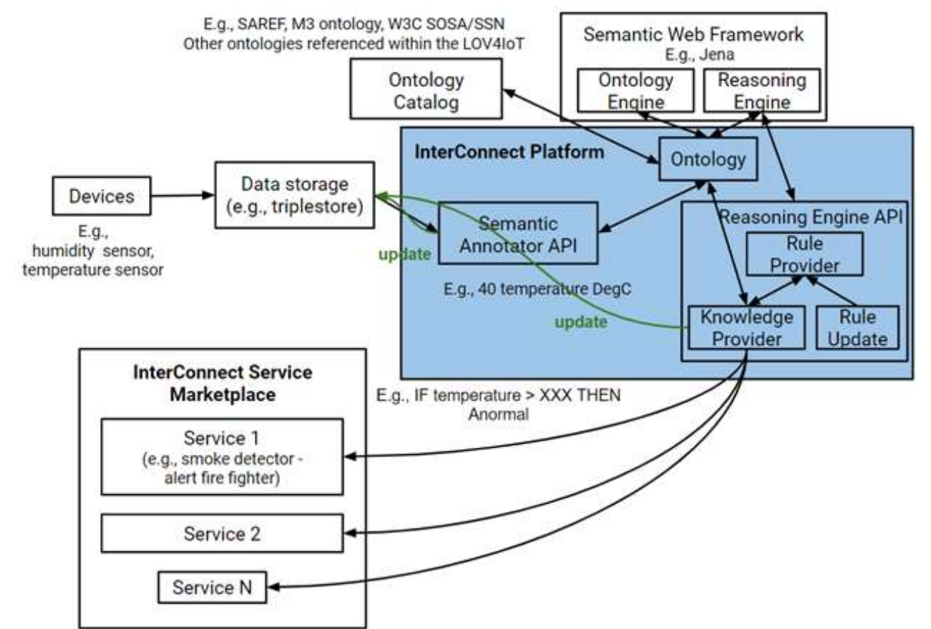
FIGURE 49 – ONTOLOGY-BASED REASONING ARCHITECTURE FROM SENSOR DATA TO END-USER SERVICES
