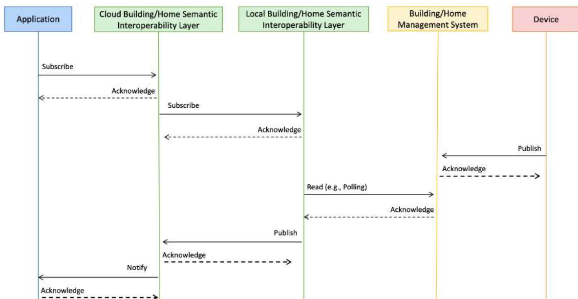
FIGURE 29 – MESSAGE FLOW EXAMPLE FOR PUBLISH/SUBSCRIPTION MESSAGING PATTERN BETWEEN ENTITIES
