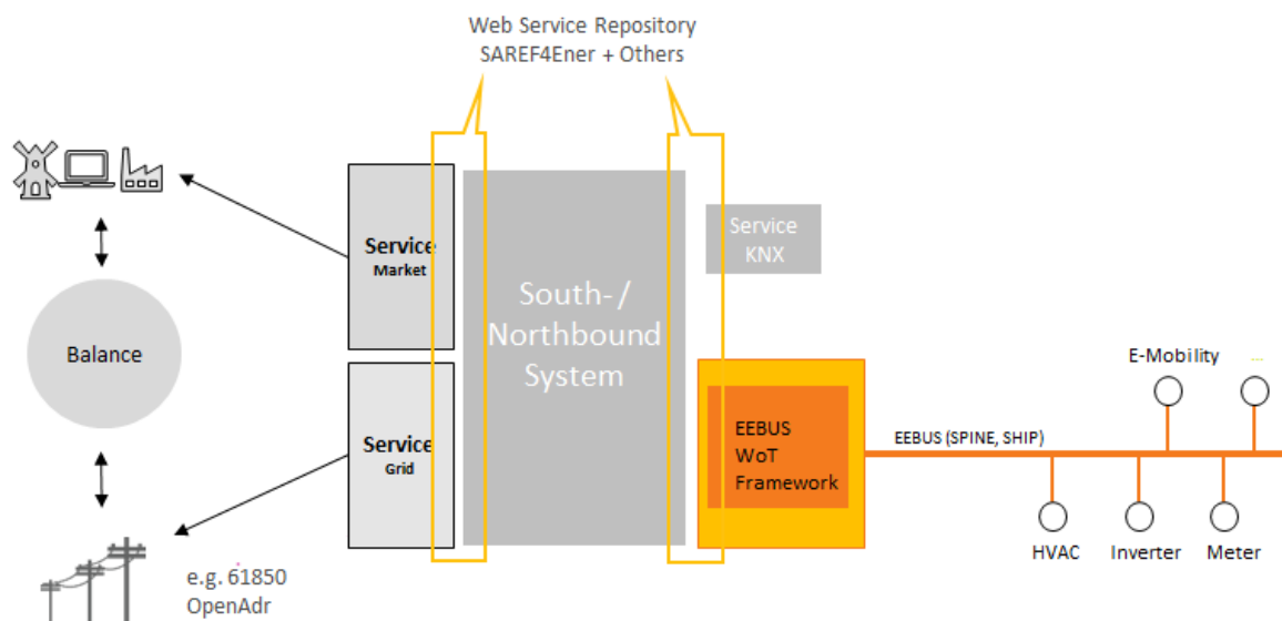
FIGURE 44 – EEBUS’S WOT FRAMEWORK
