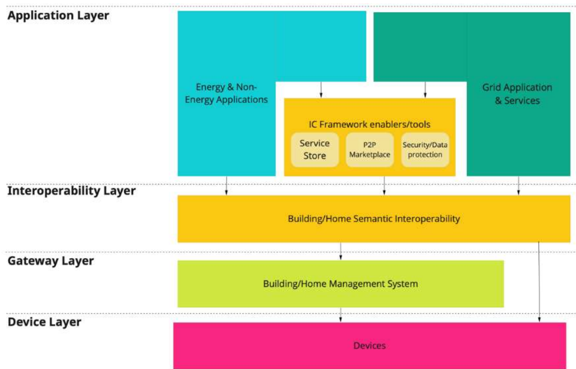
FIGURE 10 – IC’S INITIAL HIGH LEVEL REFERENCE ARCHITECTURE
