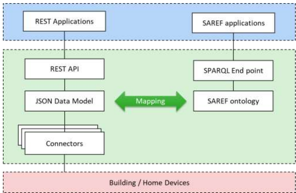
FIGURE 54 – SENSINOV’S DATA MODEL & MAPPING TO SAREF ONTOLOGY
