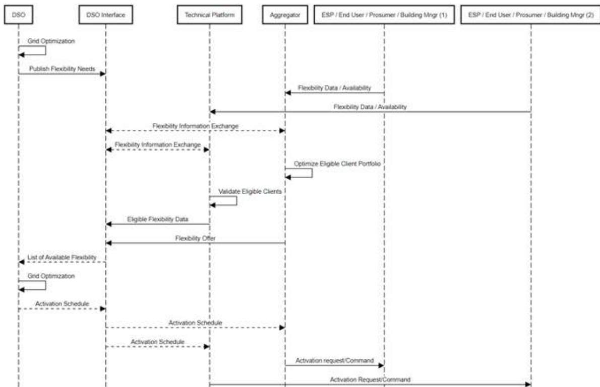
FIGURE 6 – USE CASE SEQUENCE DIAGRAM FROM THE PORTUGUESE PILOT
