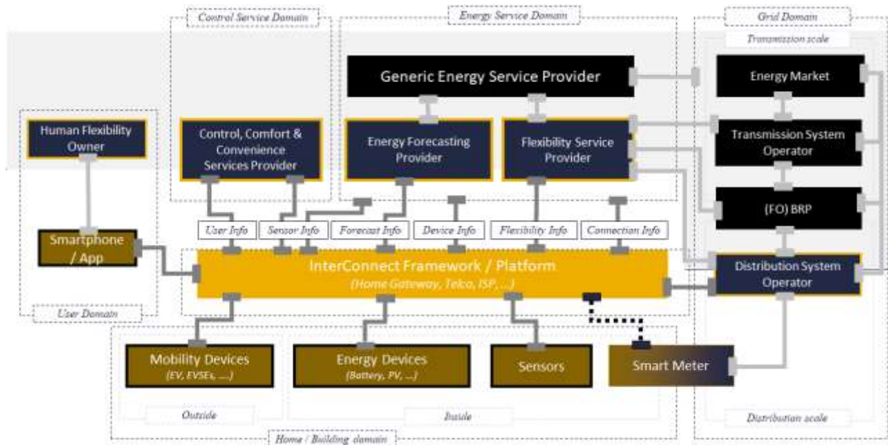
FIGURE 22 – INTERCONNECT'S SMART ENERGY REFERENCE ARCHITECTURE (SERA)
