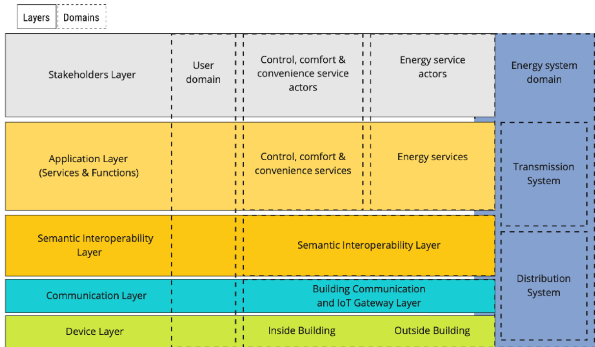
FIGURE 11 – INTERCONNECT’S SMART HOME/BUILDING AND ENERGY REFERENCE ARCHITECTURE (SHBERA)
