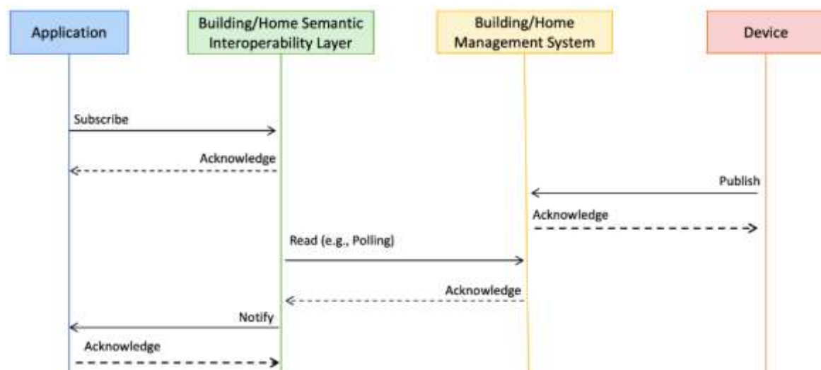
FIGURE 27 – MESSAGE FLOW EXAMPLE FOR PUBLISH/SUBSCRIPTION MESSAGING PATTERN BETWEEN ENTITIES
