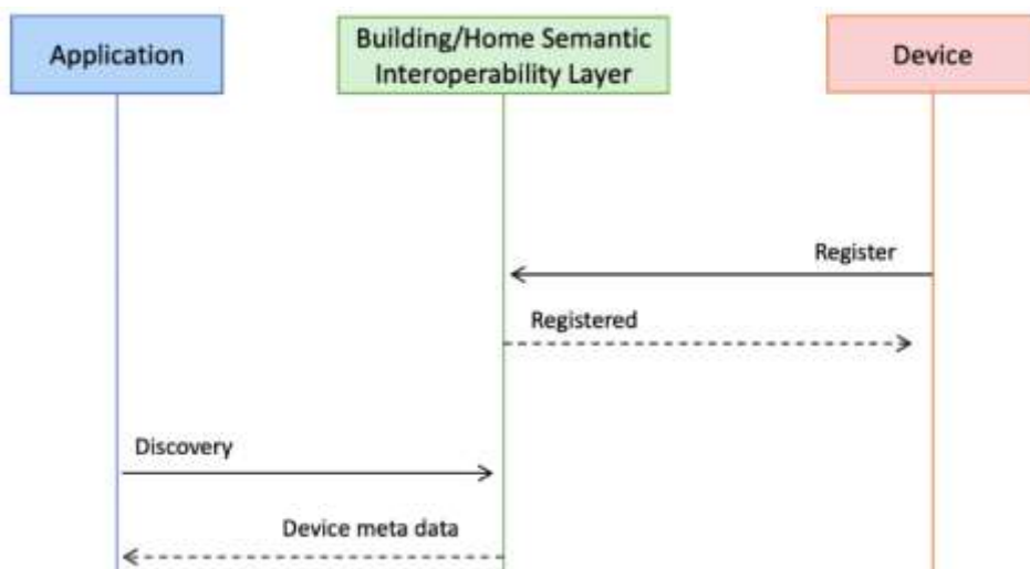
FIGURE 32 – MESSAGE FLOW EXAMPLE FOR META-DATA EXCHANGE
