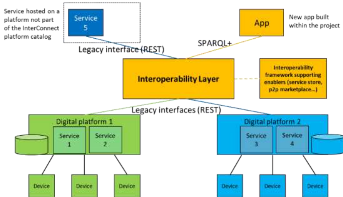
FIGURE 24 – SEMANTIC INTEROPERABILITY LAYER IN CONTEXT OF A TYPICAL PILOT ARCHITECTURE
