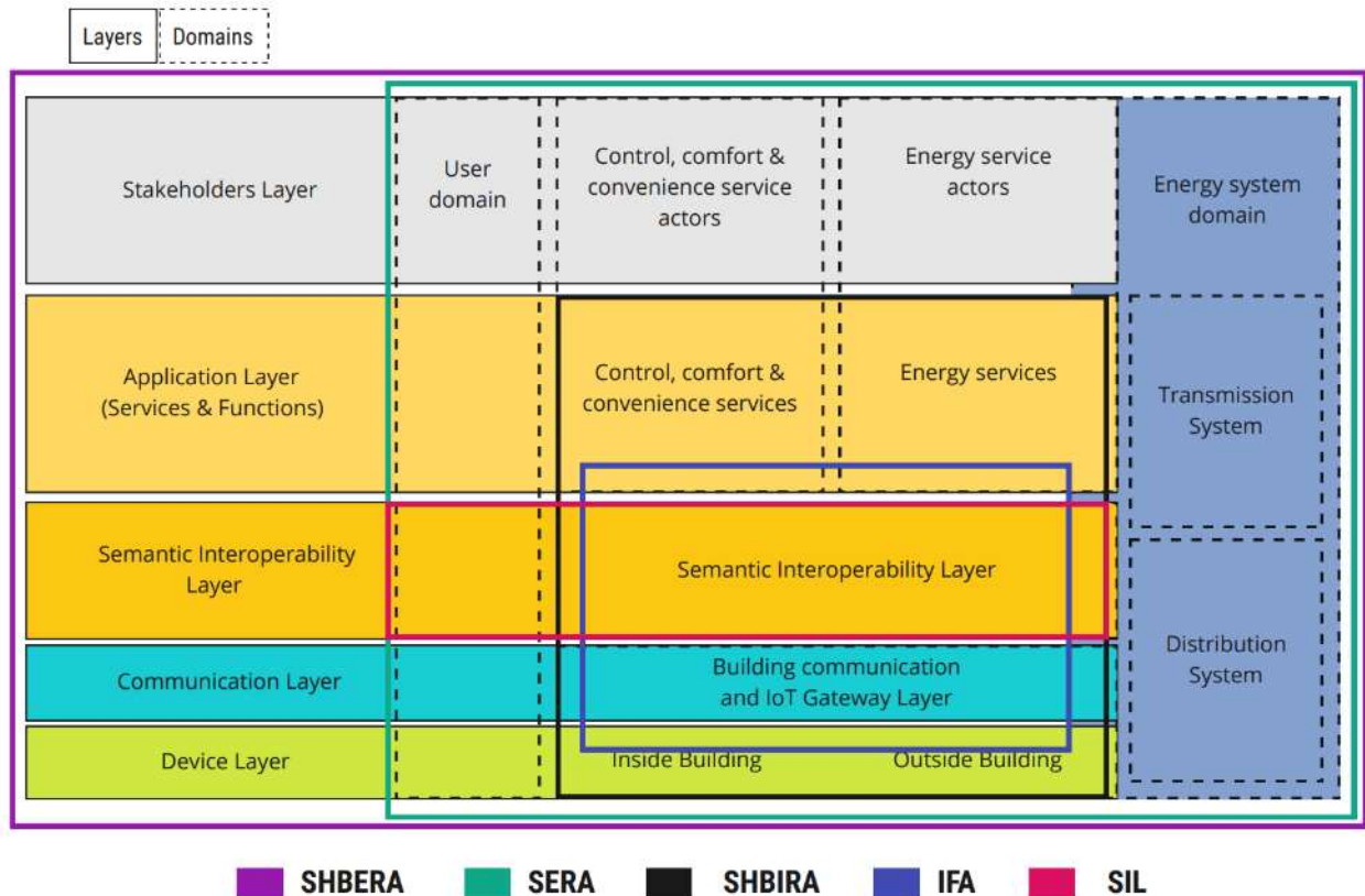
FIGURE 12 – THE SHBERA AND THE DIFFERENT ARCHITECTURAL VIEWPOINTS
