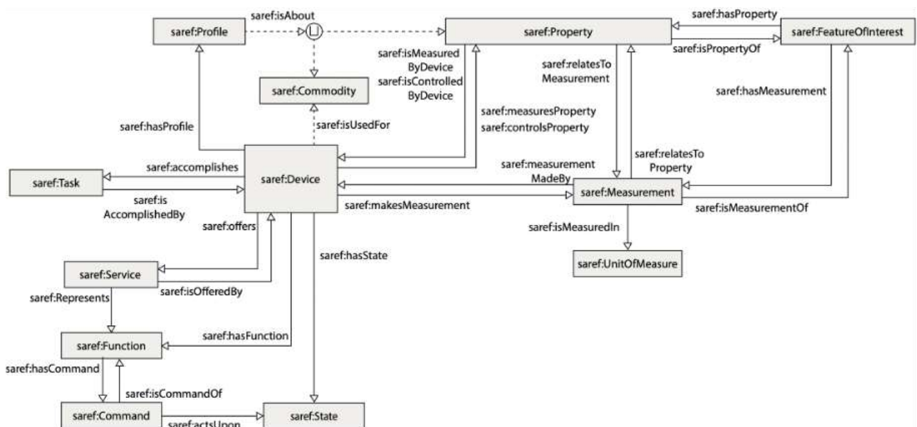
FIGURE 38 – OVERVIEW OF SAREF CORE ONTOLOGY [16]
