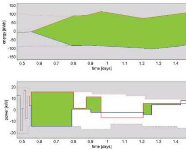
FIGURE 17 – FLEXGRAPH EXAMPLE OF A BATTERY 25
