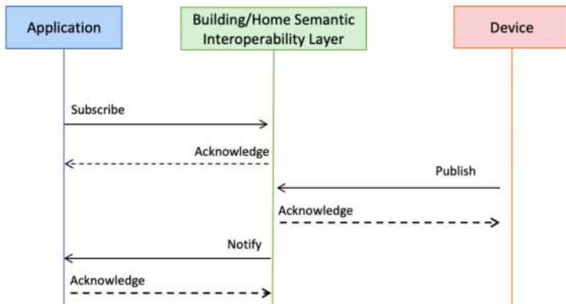
FIGURE 26 – MESSAGE FLOW EXAMPLE FOR PUBLISH/SUBSCRIPTION MESSAGING BETWEEN ENTITIES
