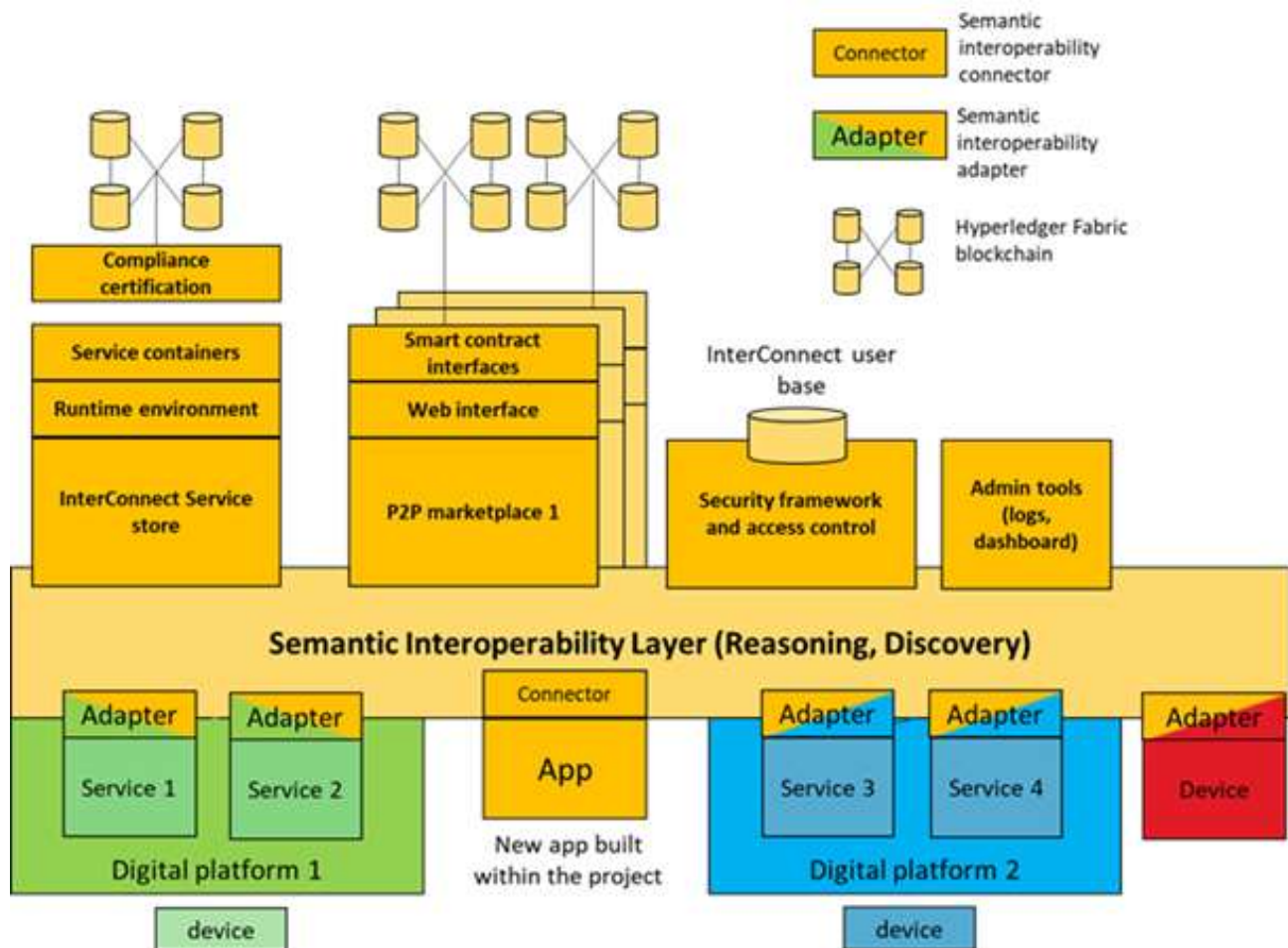
FIGURE 36 – INTERCONNECT INTEROPERABILITY FRAMEWORK ARCHITECTURE (IFA)
