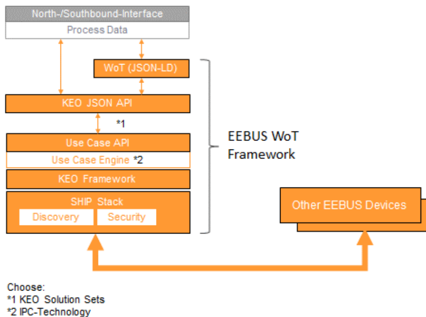
FIGURE 46 – EEBUS'S WOT FRAMEWORK
