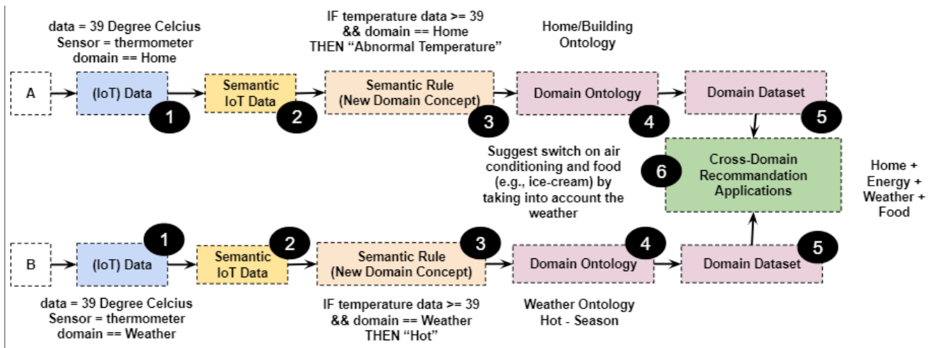
FIGURE 50 – THE IOT KNOWLEDGE-BASED CROSS-DOMAIN RULE-BASED ENGINE & DATA WORKFLOW [26]
