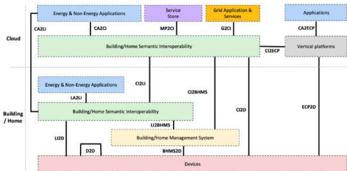
FIGURE 23 – IC'S SMART HOME AND BUILDING IOT REFERENCE ARCHITECTURE (SHBIRA)
