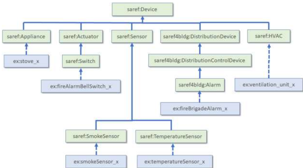
FIGURE 39 – SUBCLASS HIERARCHY OF DEVICES AND THE EXAMPLE INSTANCES. SOLID LINES DEPICT SUBCLASS RELATIONS AND DASHED LINES INSTANCE RELATIONS
