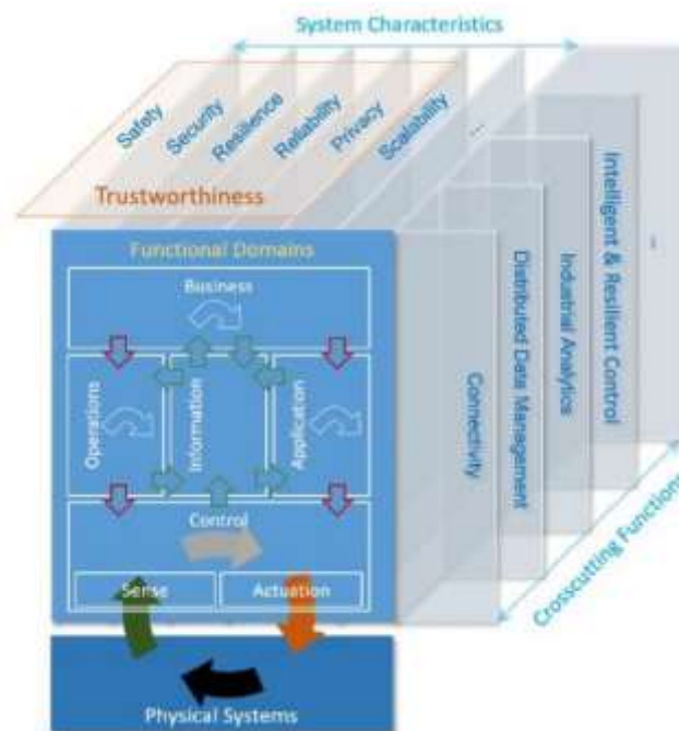
FIGURE 2 – IIRA'S FUNCTIONAL MODEL
