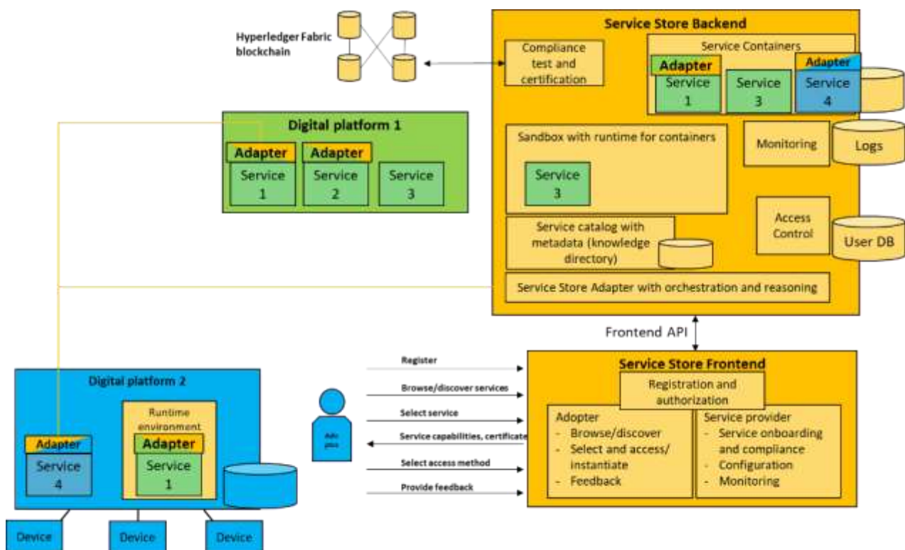
FIGURE 25 – IC SERVICE STORE FUNCTIONAL ARCHITECTURE AND FUNCTIONALITIES
